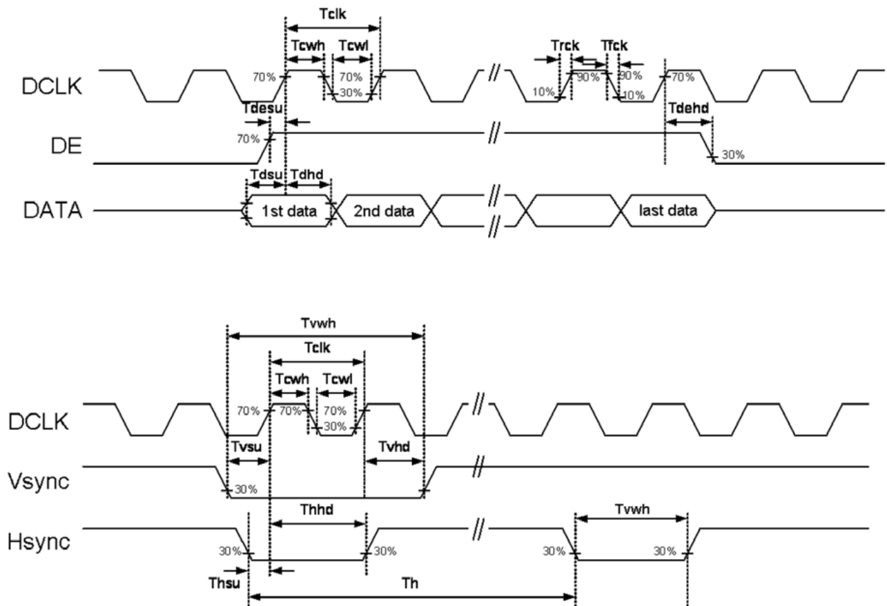
Clock and Data Input Timing Diagram
